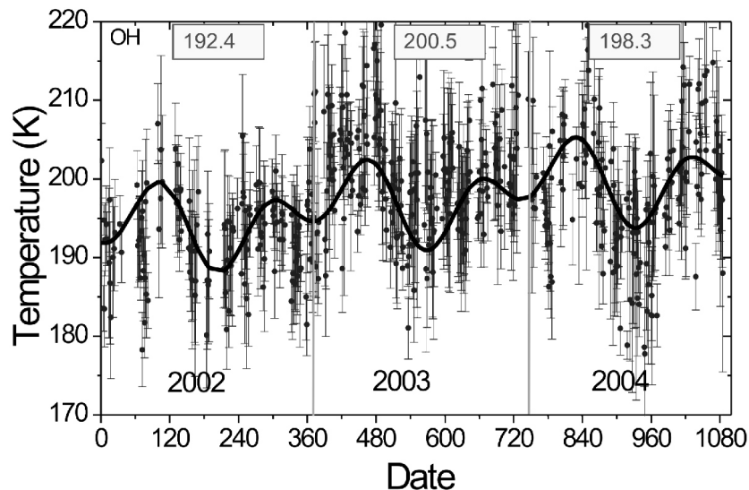
Figure 8 – Plot of nightly averaged OH rotational temperatures for three consecutive years 2002-2004. (Note, only data >4 hours in duration are shown). The data show evidence of a semi-annual oscillation as well as an annual oscillation as expected from this low-latitude site but rarely measured to date.
