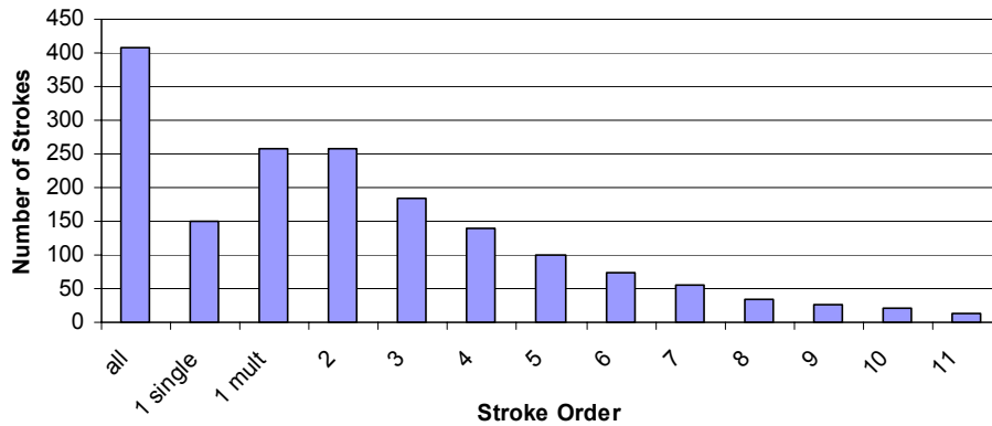
Fig. 4.1: Number of negative CG strokes for each stroke order of the FM data
