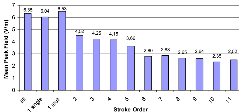
Fig.4.2: Mean peak value normalized to 100 km in V/m versus stroke order of CG strokes of FM data
