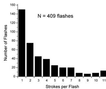
Fig. 3.2: Number of strokes per flash
