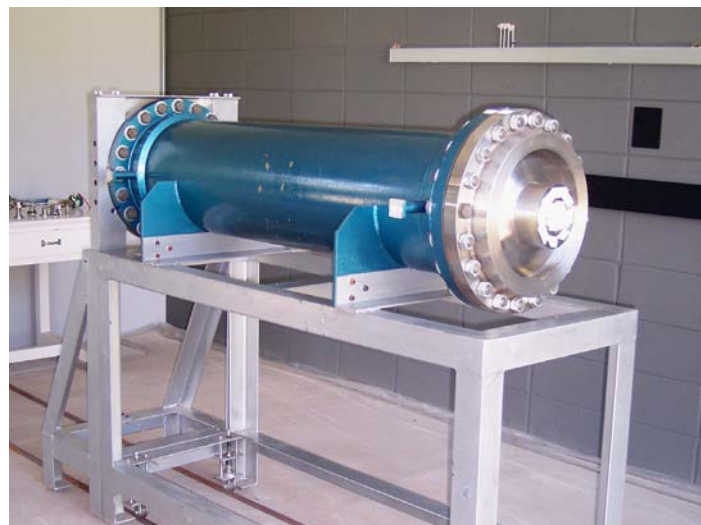
Figure 5: The new vitiated air generator (Leite, 2006).
