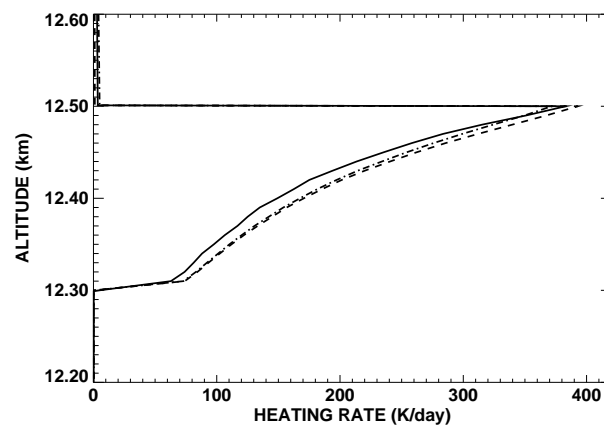
Figure 2: The same but for high cloud layer at the height from 12.3 km to 12.5 km.
