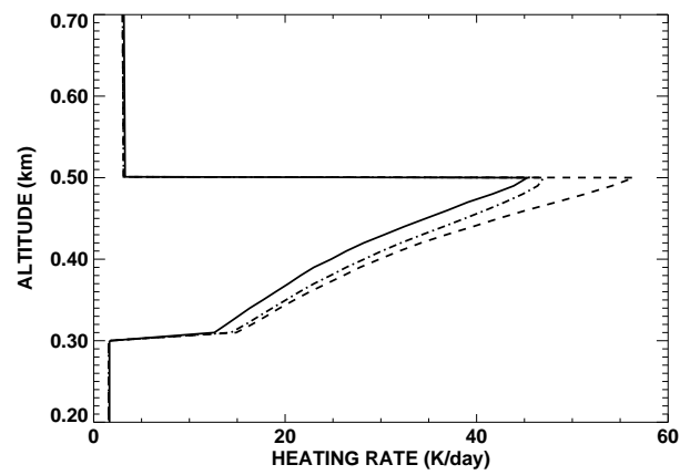
Figure 1: Heating rates inside low cloud layer at the height from 300 m to 500 m ( R_{\text{eff}}=31\mu\text{m} , \text{COD}=48.5 , \text{SZA}=30^\circ , MLS atmosphere) calculated by FLBLM (solid), MKD (dashed), and MKD with the correlation treatment (dot-dashed).
