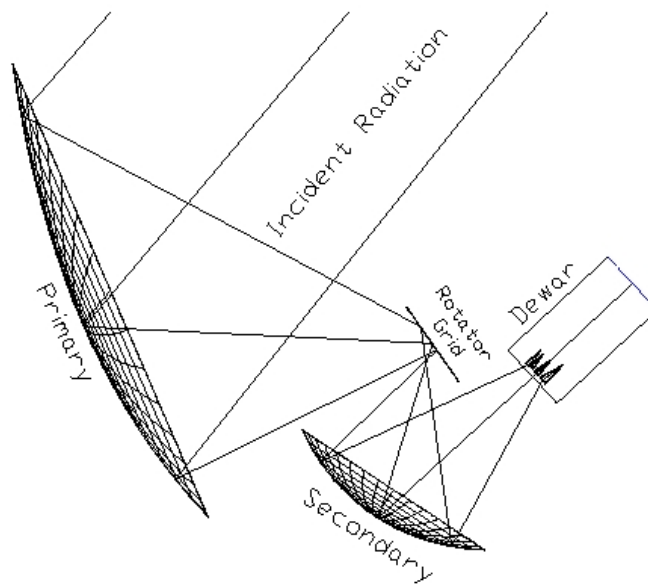
Fig. 1. Optical schematic for COFE and B-machine prototype telescopes, an off-axis Gregorian configuration optimized for minimal cross-polarization contamination. A 2.2 m parabolic reflector primary, a 0.9 m ellipsoidal secondary, and a 0.3 m rotator grid are shown.
