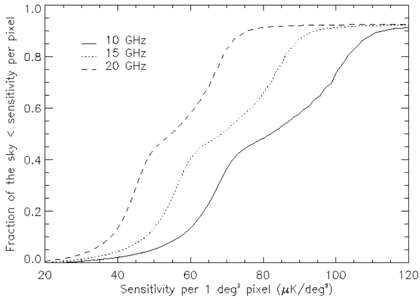
Fig. 8. Integrated histogram of anticipated aggregate sensitivity per 1 deg 2 pixel assuming a 24 hour flight from the Northern Hemisphere (Fort Sumner, NM) and a 24 hour flight from the Southern Hemisphere (Alice Springs, Australia). For each COFE band, we plot the fraction of the entire sky measured with better than a given aggregate sensitivity. The change of the curves slope is due to the fact that 35% of the sky can be observed from both hemispheres using COFE scan strategy.
