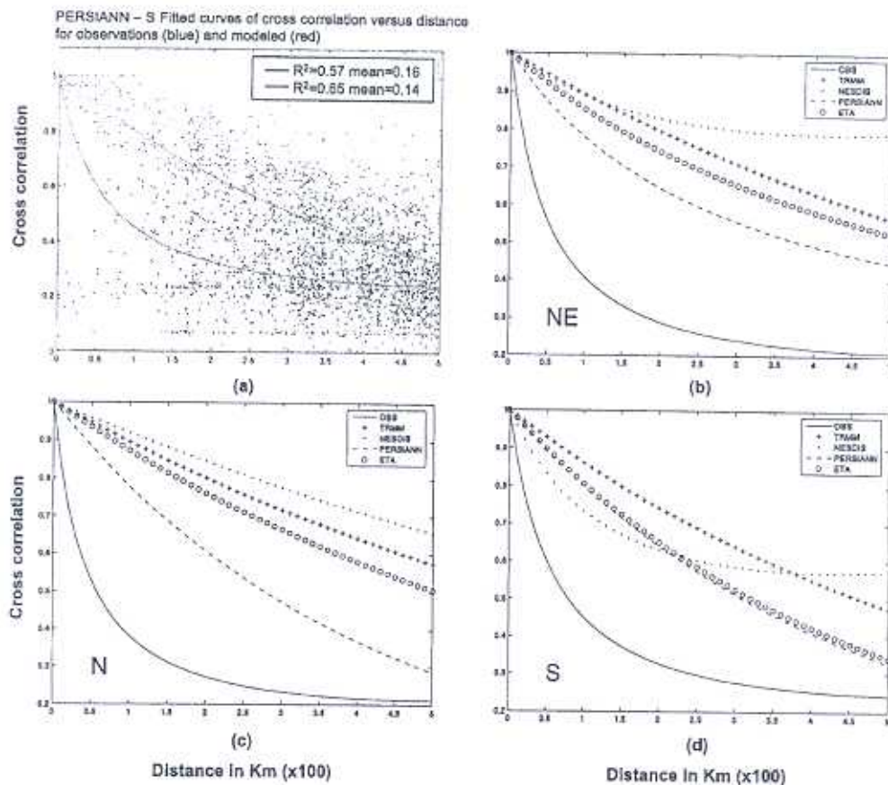
Figure 6. Cross-correlation coefficient versus distance for each valid location within each region: (c) north, (b) northeast, and (d) south. (a) Example of the data distribution and the fitted curve for PERSIANN and observations. The x axis represents the distance in hundreds of kilometers, and the y axis represents the cross-correlation coefficient.
