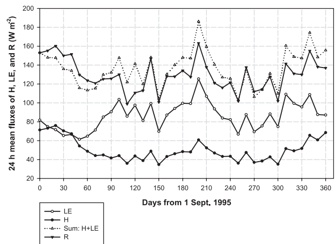
Figure 7. Fluxes summed over the full 24 hour cycle, and shown as ten-day means: sensible heat flux, H , latent heat flux, LE and net radiation, R , with gap-filled values of H and LE being used where field data do not exist. The gap-filling procedure is described in the text.
