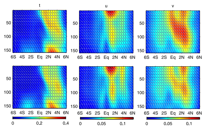
Figure 3. First and second row show the variability of the CTL and STD experiments, respectively, averaged over 150°W to 90°W. The standard deviation of T is on the left (°C), of u in the central column and of v on the right ( \text{m s}^{-1} ).
