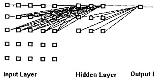
Fig. 2 — Architecture for a single hidden layer Time Delay Neural Network.
