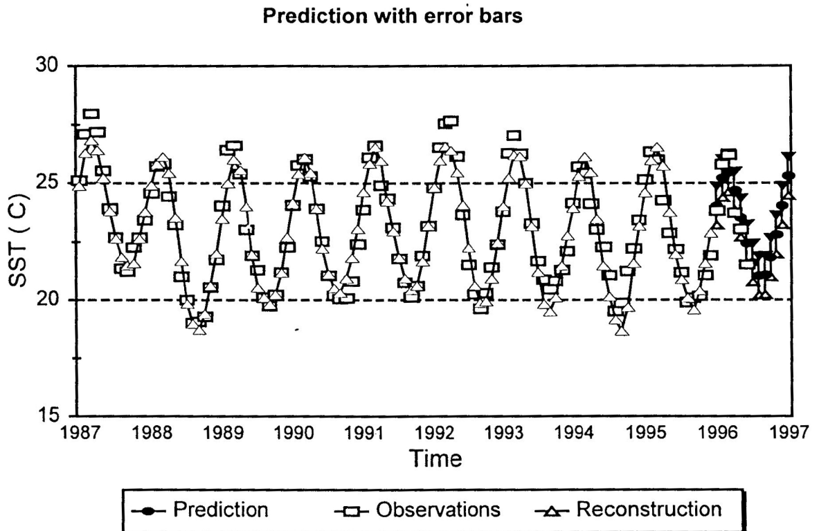
Fig. 4 — Reconstruction and prediction of SST in the region Niño1-2 using Time Delay Neural Networks.
