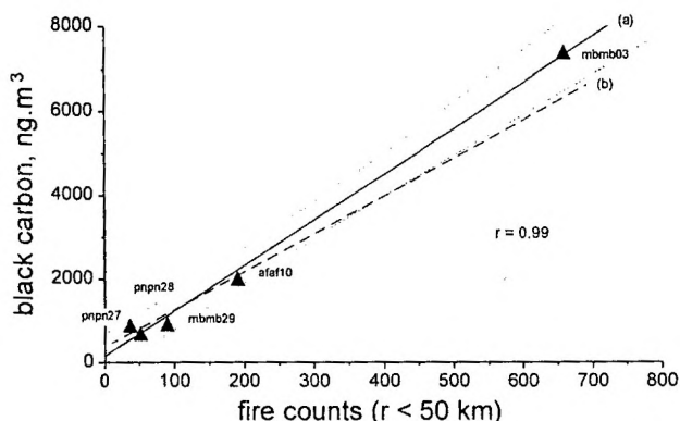
Figure 6. AVHRR/NOAA fire spot counts for 50-km radius circle of investigation versus black carbon for the vertical profile flights. The correlation coefficient is high and the adjusted straight line (solid line) through the points is shown along with the 95% confidence level (dotted lines). A second regression line (dashed line) is also adjusted through the points but excluding the very high MBMB03 data point.
