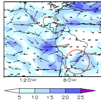
Figure 5.11. February 2005 200 hPa wind anomaly. Source: CPTEC/INPE.
