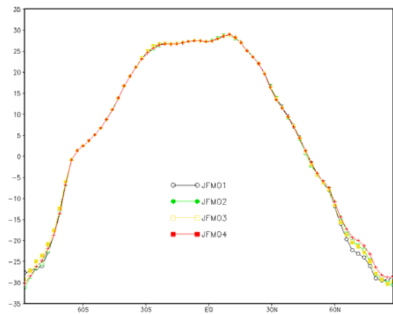
Figure 4.2. b) Average zonal distribution of air temperature on the surface in °C (TS), for the months of January to March.
