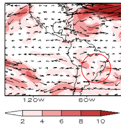
Figure 5.12. February 2005 850 hPa wind anomaly Source: CPTEC/INPE.
