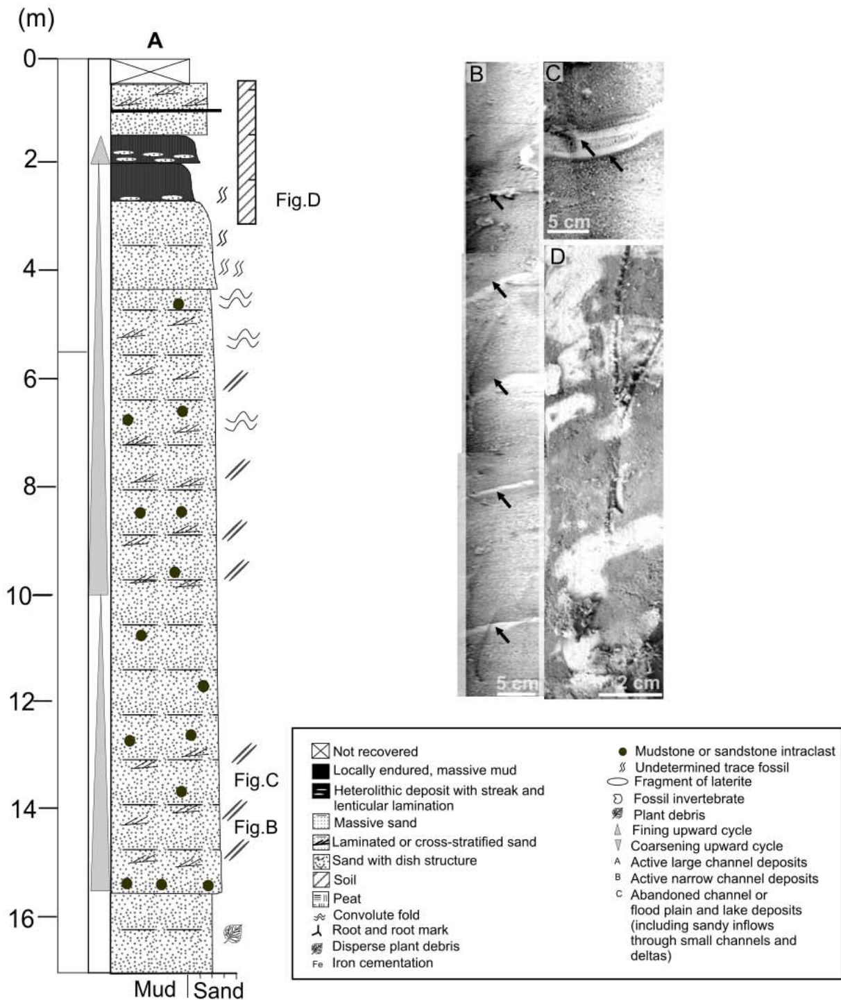
Fig. 3 – Drill #1 (main channel to the north). A) Lithostratigraphic profile illustrating facies characteristics and vertical facies distribution. B) Cross stratified sands with foreset packages marked by reactivation surfaces and/or mud drapes (arrows). C) Detail of a cross set displaying mud couples (arrows) that define thicker/thinner sand packages, attributed to ebb/flood tidal fluctuation. D) Mottled muddy deposits from the top of the main fining upward succession, recording deposition from suspension during channel abandonment. Mottling is probably related to root development (See Figure 2 for drill location).
