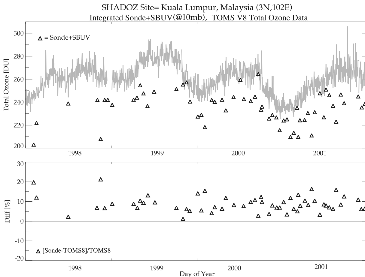
Figure 7e. Same as Figure 7a except for Kuala Lumpur, Malaysia.
