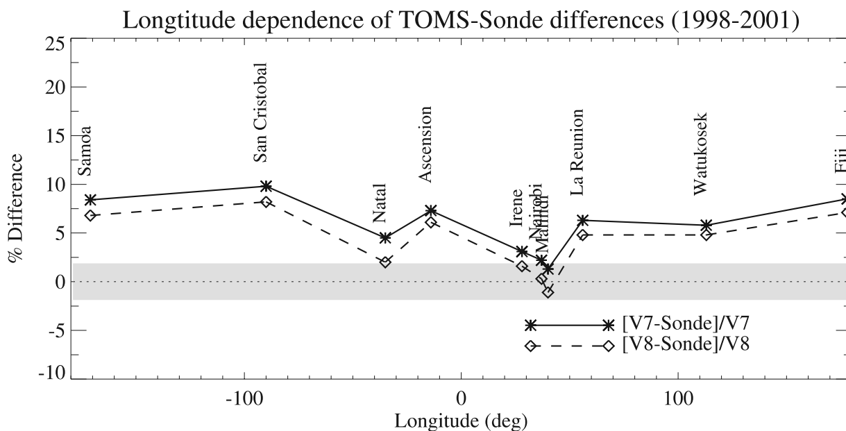
Figure 8. Summary of averaged differences between total O 3 from SHADOZ sondes and from TOMS (v 7 [cf. Thompson et al. , 2003a, Figure 9]) and sondes and TOMS v 8. Data to 10 hPa (Table 4) with SBUV extrapolation are used for sonde total ozone. Shaded region corresponds to “best total ozone” based on Dobsons and most recent TOMS calibration.
