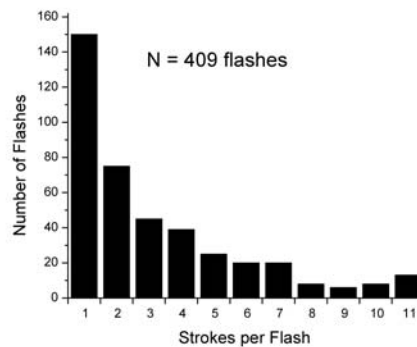
Fig. 3.2: Number of strokes per flash
