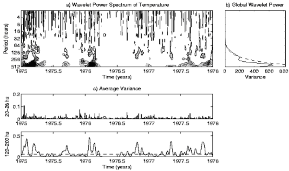
Fig. 7: Same as in Fig. 6, but for the SST time series ( \sigma^2=10.4^\circ\text{C}^2 ), with the shaded contours in (a) being at normalized variances varying from 40 to 120 with interval of 40.
