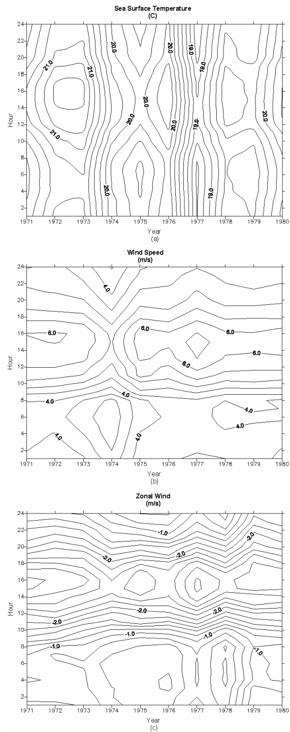
Fig. 5: Hourly mean values of: a) SST ( ^{\circ}\text{C} ), b) wind speed, and c) zonal wind component ( \text{m s}^{-1} ) for each year. The values of SST and wind correspond to an average over the twelve calendar months.
