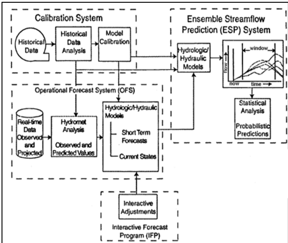
Figure 64. Schematic representation of the National Weather Service River Forecasting System (NWSRFS).
