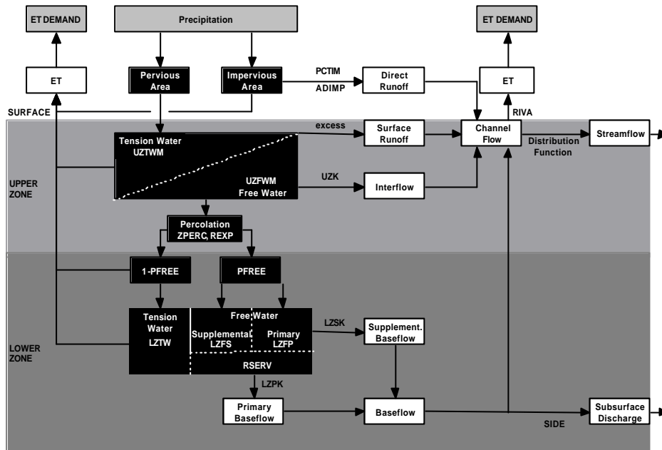
Figure 65. Sacramento Soil Moisture Accounting Model (SAC-SMA).
