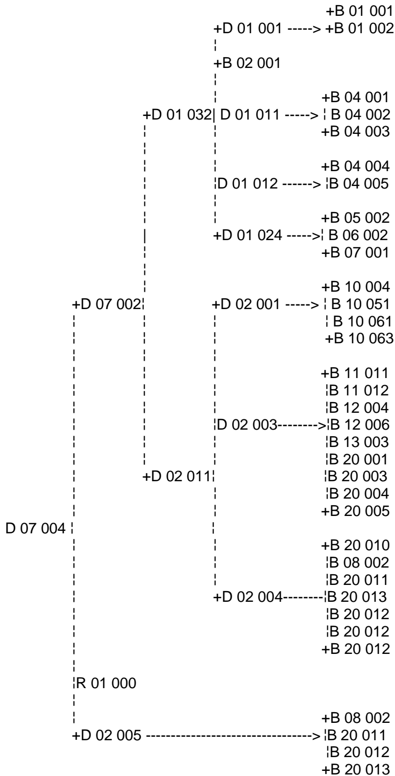
Figure 3.2.4-5: Level 4 Decomposition of the Basic Sequence Descriptor from the Sample CREX Message
