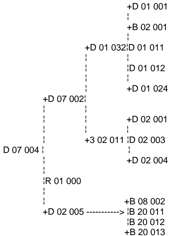
Figure 3.2.4-4: Level 3 Decomposition of the Basic Sequence Descriptor from the Sample CREX Message
