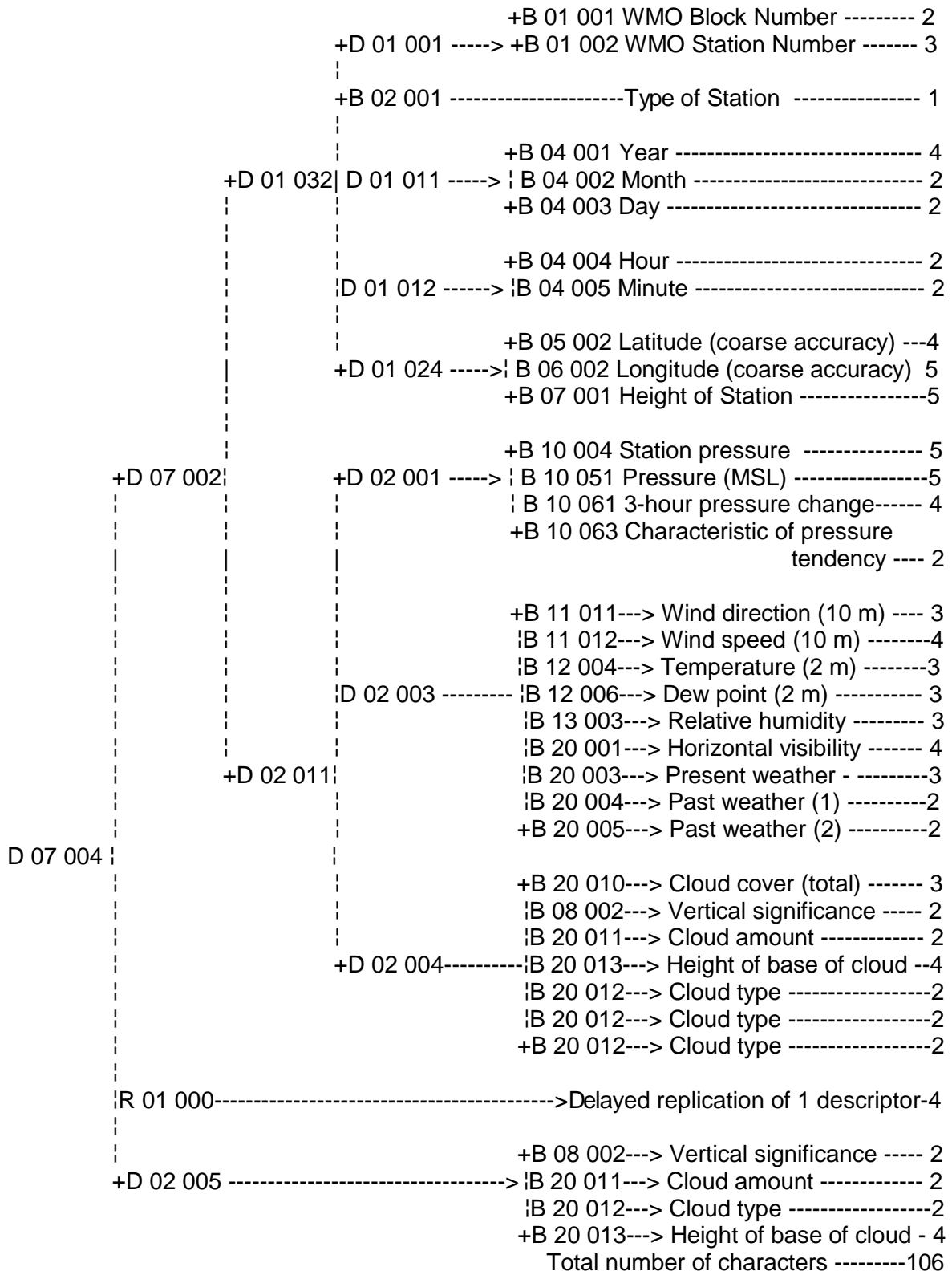
Figure 3.2.4-6: Level 5 Decomposition of the Basic Sequence Descriptor from the Sample CREX Message
