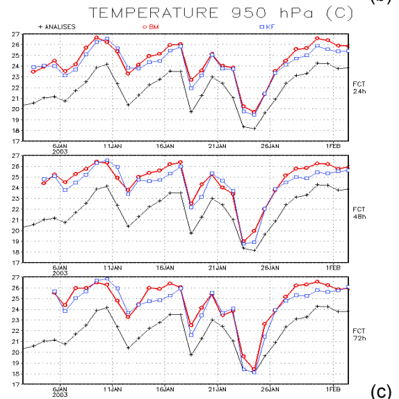
Fig.7: Timeseries of spatial average of precipitation(a), SLP(b) and temperature at 950 hPa(c) for the area (35S-20S and 67.5W-55W). Betts-Miller scheme (red) and Kain-Fritsch scheme (blue).
