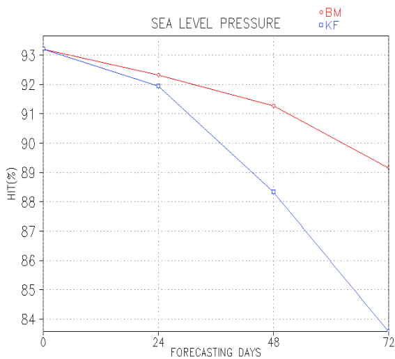
Fig. 6: Hit rate of sea level pressure with Betts-Miller scheme (red) and Kain-Fritsch scheme (blue).
