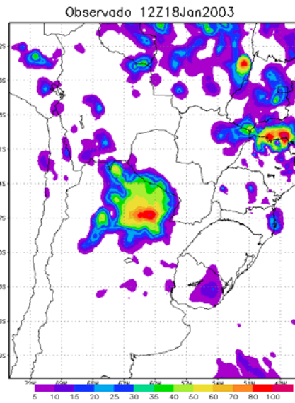
Fig.11: 24 hour observed precipitation (mm) valid for 18/01/2003 12Z .
