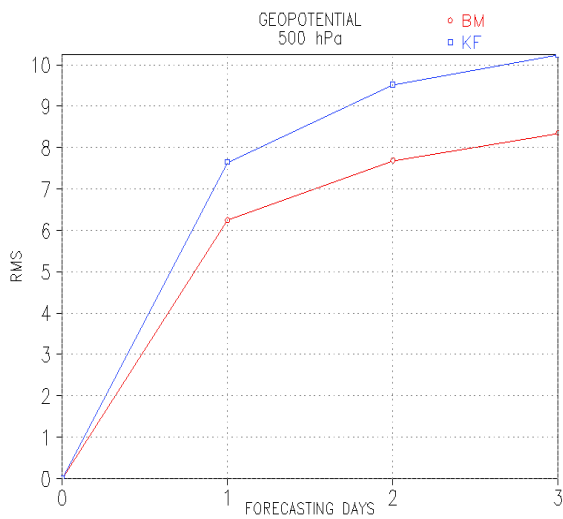
Fig.5: Root Mean Square (rms) of geopotential at 500 hPa with Betts-Miller scheme (red) and Kain-Fritsch scheme (blue).
