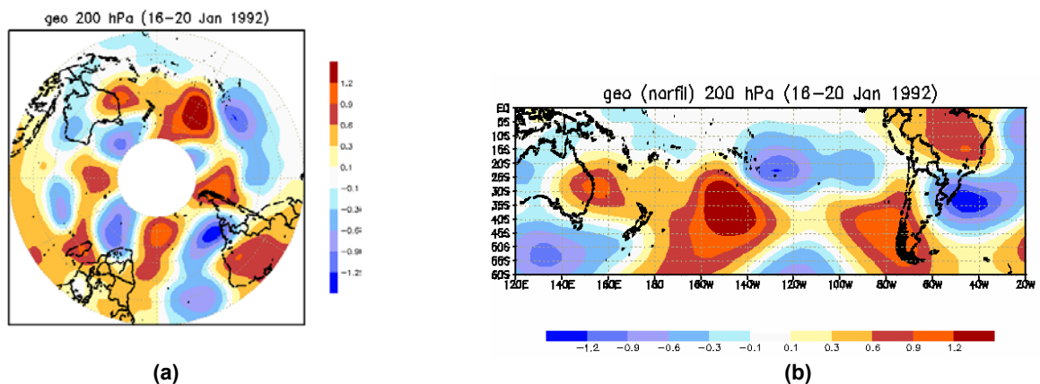
Fig.5-Averaged 200 hPa geopotential intraseasonal filtered anomalies for the period of January 16 th to 20 th , 1992 (reanalysis). (a) polar stereographic view; (b) Lat X Lon view.
