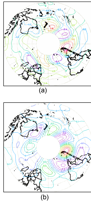
Fig.4- Anomaly correlations of 200 hPa geopotential of grid point 80°W, 45°S with all the other grid points (a) reanalysis; (b) CPTEC/COLA AGCM.
