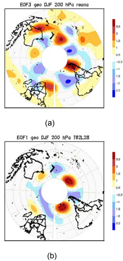
Fig.2- EOF of geopotential at 200 hPa in DJF. (a) EOF3 reanalysis; (b) EOF1 model results.
