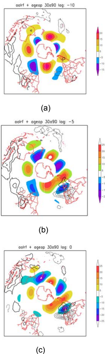
Fig.1- Composite of observed anomalous OLR and geopotential at 200 hPa for summer periods with filtered 30-90 days negative anomaly OLR in SACZ region, greater than one standard deviation. (a) Lag -10, (b) Lag -5, (c) Lag 0.
