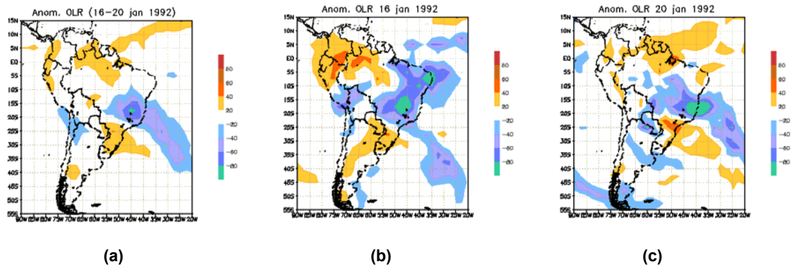
Fig. 6- Daily OLR anomalies (unfiltered ) (a) Mean January 16 th to 20 th , 1992; (b) day 16 th ; (c) day 20 th . (observations)
