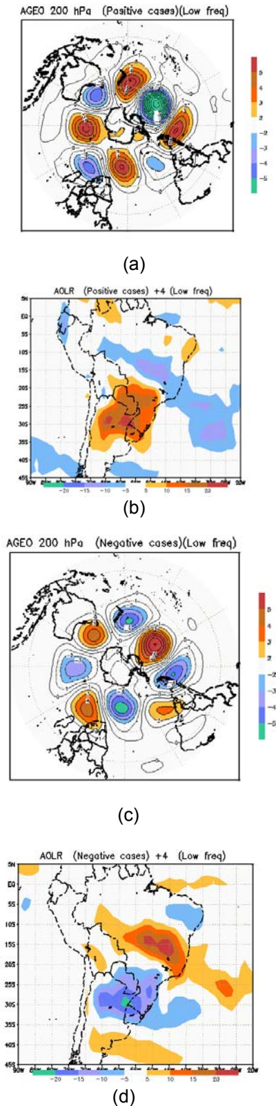
Fig.3- Composite of cases with extreme wave 4 amplitude in the model results (a) case 1 : 200 hPa geo.anom.; (b) case 1 : OLR anomaly four days later; (c) case 2: 200 hPa geo. anom.; (d) case 2: OLR anomaly four days later.
