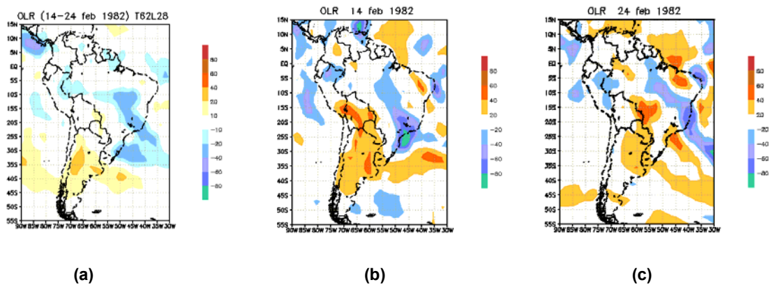
Fig. 8- Daily OLR anomalies (unfiltered) (a) Mean February 14 th to 24 th , 1982; (b) day 14 th ; (c) day 24 th . (Model)
