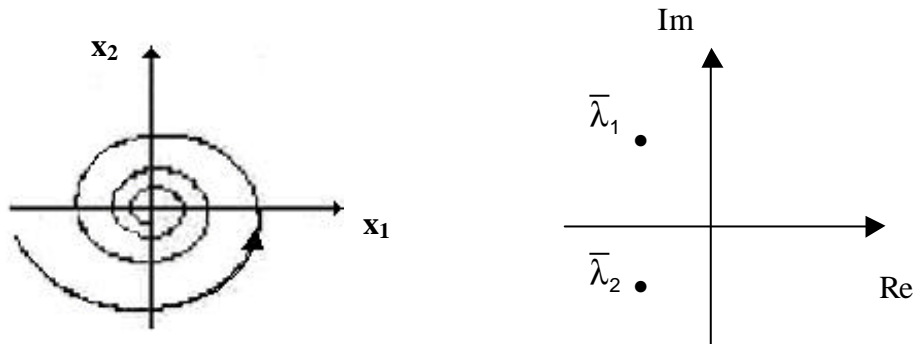
FIGURA 3.7 – Diagrama de fase para \bar{\lambda}_{1,2} = \hat{\alpha} \pm \hat{\beta}i , \hat{\alpha} < 0, \hat{\beta} > 0 .
