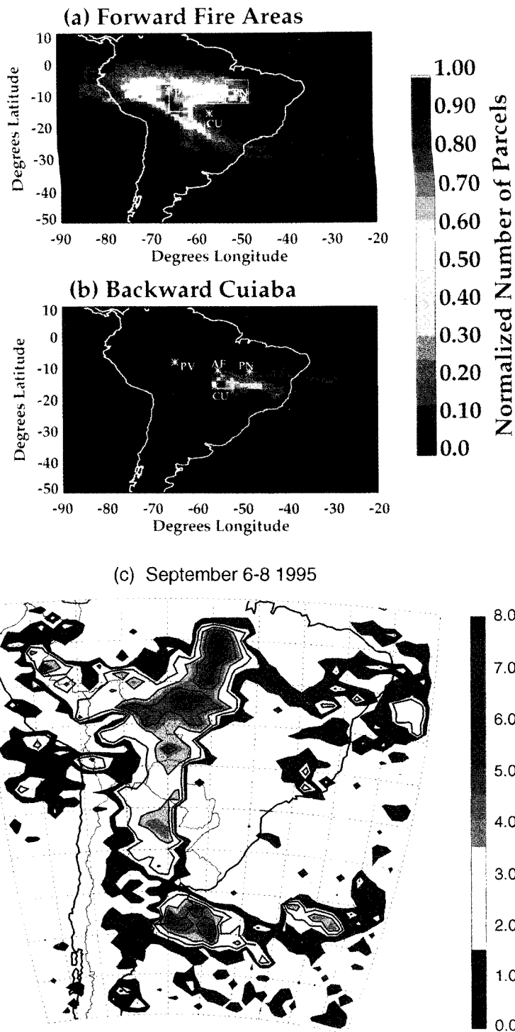
Plate 3. Hourly air parcel locations along (a) 6 day forward trajectories originating from the main biomass burning areas and (b) along 6 day backward trajectories starting from a cluster of points near Cuiabá ( 16^{\circ}\text{S} , >56^{\circ}\text{W} ). Starting levels are \sim 700 mbar. The trajectory starting points in Plate 3a are distributed according to the main biomass burning areas observed during the experiment from the GOES-8 fire product [Prins et al. , this issue]. The trajectories are three-dimensional cinematic calculated from the University of São Paulo model [Freitas et al. , 1996] using simulated wind fields with 80 km resolution. (c) Example of GOME data from September 6 to 8, 1995, during the SCAR-B experiment showing the transport of smoke to the Atlantic Ocean. Heavy clouds associated with the transport reduce the ability of satellites to observe it. In this case, 10% of the smoke detected by GOME is over the ocean.
