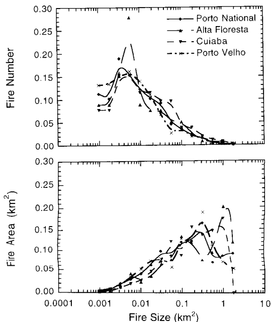
Figure 8. Histograms of the fire size distribution for four locations in Brazil sampled by the MAS instrument on the ER-2 in SCAR-B. Fires are detected using the 3950 nm channel (fire pixel is detected for apparent temperature at 3950 nm > 335 K). (top) The distribution of number of fires as a function of the fire size. (bottom) The distribution weighted by the fire area. All the distributions are normalized to a total probability of 1.0 (data from Kaufman et al. [this issue]). Note that the fire size is defined here by the MAS 50 m pixels that have an average apparent temperature at 3950 nm > 335 K.
