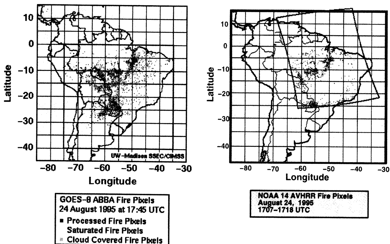
Plate 5. Example of fire detection from satellites by GOES-8 (4 km resolution 3950 nm channel) and AVHRR (1 km resolution 3750 nm channel). (a) The GOES-8 fire product at 1745 UTC on August 24, 1995, one of the peak burning days during SCAR-B, showing the locations of over 4400 fires detected with the GOES-8 ABBA algorithm. The red markers indicate fires that were processed by the GOES-8 ABBA providing estimates of subpixel fire size and temperature; yellow indicates saturated fire pixels; and blue represents cloud-covered fire pixels. (b) NOAA-14 advanced very high resolution radiometer (AVHRR) local area coverage (LAC). The red dots indicate the fire pixels, and the region enclosed in blue is the area covered by the NOAA-14 AVHRR for this day between 1707 and 1718 UTC.
