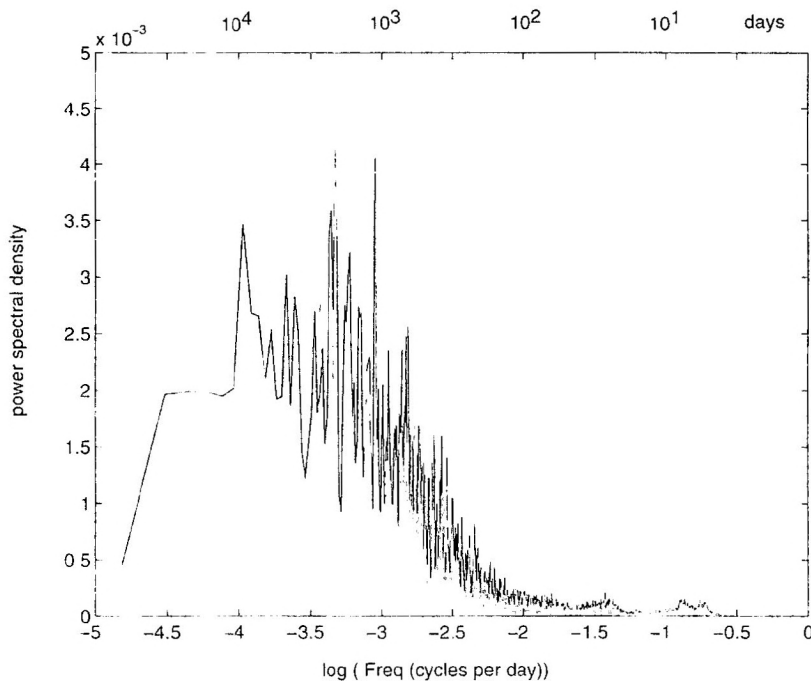
Figure 12. Run 2: Power spectrum P_\alpha as a function of the logarithm of frequency computed from 400,000 days of \alpha for m = 2 , n = 5 , N = 3 , h = 2500 m, and Ro_T = 0.07 ( 70^\circ\text{C} ) with seasonal forcing. The power spectrum is shown by the bold black line, and the half width of the 95% confidence interval is shown by the thin gray line.
