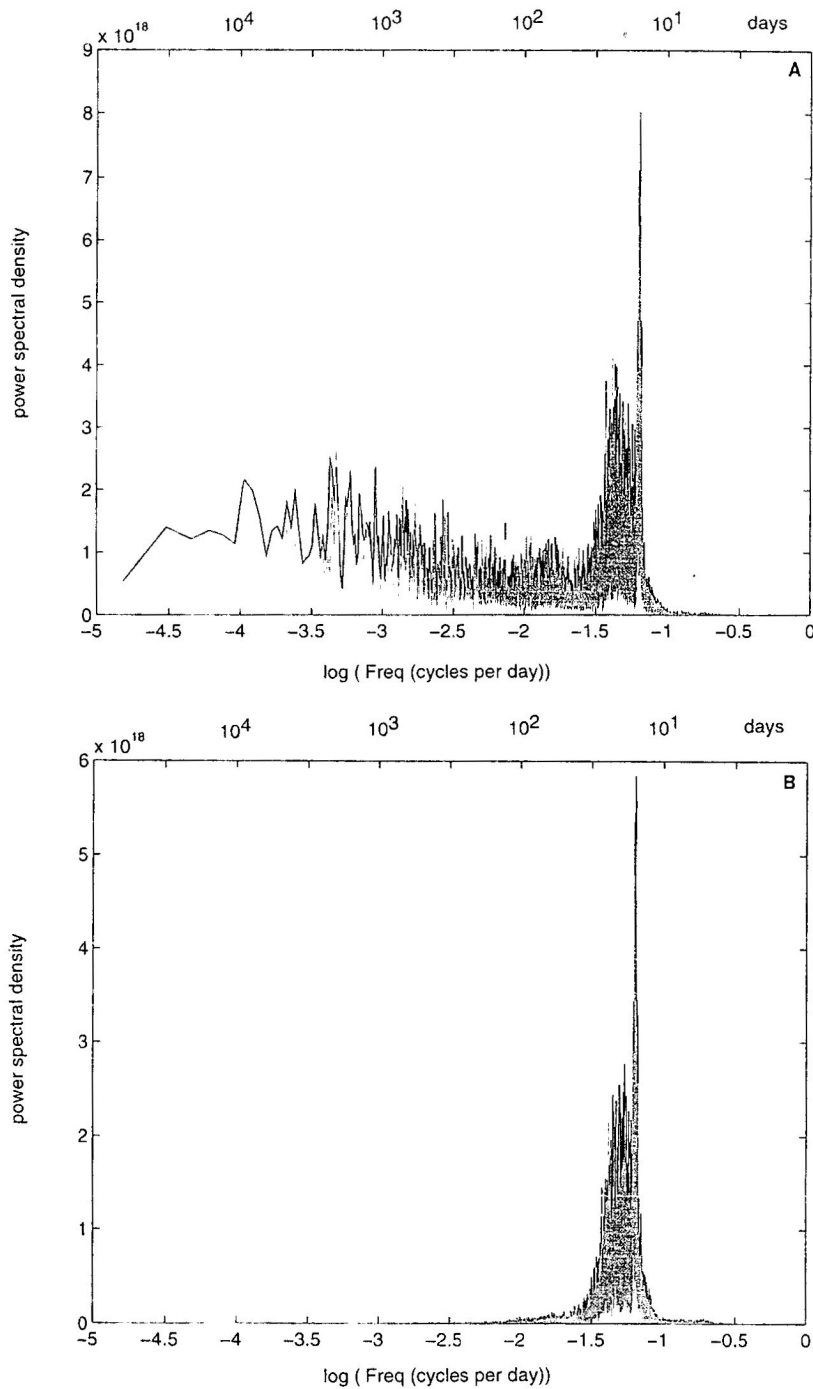
Figure 14. Run 2: Power spectrum of (a) PC 1, (b) PC 2, (c) PC 3, and (d) PC 4. Notation as in Figure 12.
