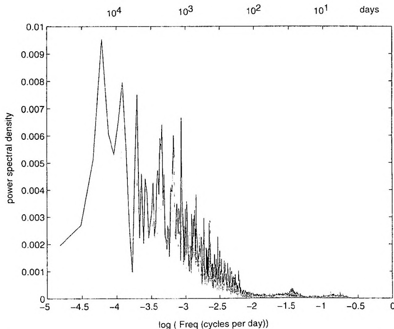
Figure 8. Run 1: Power spectrum P_\alpha as a function of the logarithm of frequency computed from 400,000 days of \alpha for m = 2 , n = 5 , N = 3 , h = 2500 m, and Ro_T = 0.07 ( 70^\circ\text{C} ) without seasonal forcing. The power spectrum is shown by the bold black line, and the half width of the 95% confidence interval is shown by the thin gray line.
