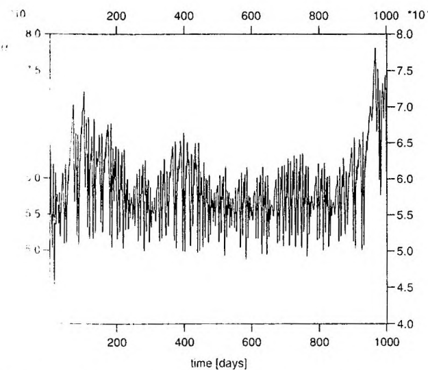
Figure 4. Temporal evolution of \alpha(t) in the chaotic regime (B) for m = 2 , n = 5 , N = 3 , h = 2500 m, and Ro_T = 0.07 (7°C), for the first 1000 days of integration.
