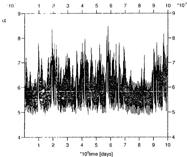
Figure 7. Temporal evolution for the first 10,000 days of integration of the zonal index \alpha(t) in the chaotic regime for m = 2 , n = 5 , N = 3 , h = 2500 m, and Ro_T = 0.07 ( 70^\circ\text{C} ).
