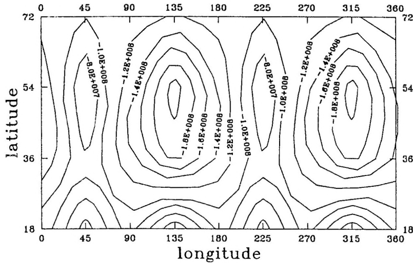
Figure 11. Run 2: Climatology of the stream function \psi ( \text{m}^2/\text{s} ) for m = 2 , n = 5 , N = 3 , h = 2500 m, and Ro_T = 0.07 ( 70^\circ\text{C} ) with a seasonal cycle.
