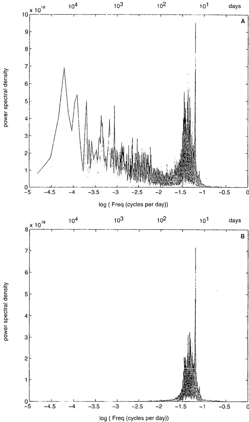
Figure 10. Run 1: Power spectrum of (a) PC 1, (b) PC 2, (c) PC 3, and (d) PC 4. Notation as in Figure 8.
