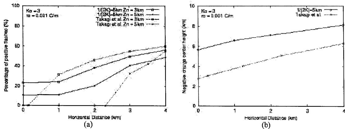
Fig 2 – (a) Percentage of positive flashes with constant conductivity profile and an exponentially increasing conductivity profile with height (dotted line). (b) The upper bound limit for positive discharge considering the horizontal displacement between opposite charge centers.
