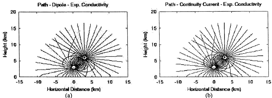
Fig. 1 – Simulated path taking into account (a) the dipole model and (b) the continuity current model.
