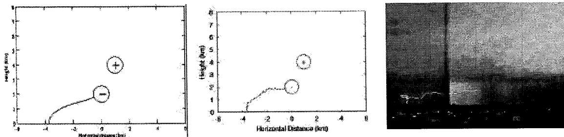
Fig. 3 – A long horizontal discharge: (a) a simulated path in a standard atmosphere, (b) a simulated path in a locally disturbed atmosphere, and (c) a natural discharge.
