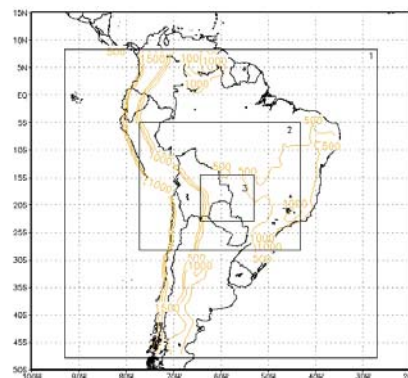
Figure 1 BRAMS nested grids considered in the simulations. Contours correspond to terrain elevations of 500, 1000 and 1500 m.
