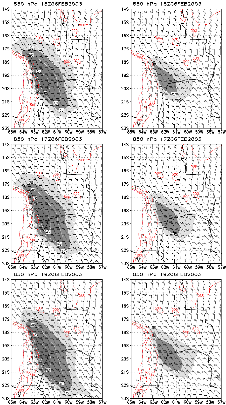
Figure 3 Comparison between the wind fields at 850 hPa obtained in the BRAMS finer resolution grid with sigma-z (left) and shaved-eta (right) vertical coordinates. ( shaded : wind strength greater or equal to 30 kt, each 5 kt; 1 full barb = 10 kt). Fields in mountain areas higher than 1500 m are masked.
