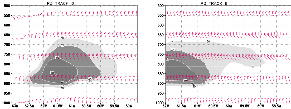
Figure 4 Isotach analysis (kt) and horizontal wind ( shaded : wind strength greater or equal to 30 kt, each 5 kt; 1 full barb = 10 kt) in vertical cross sections along transects 6 and 9.
