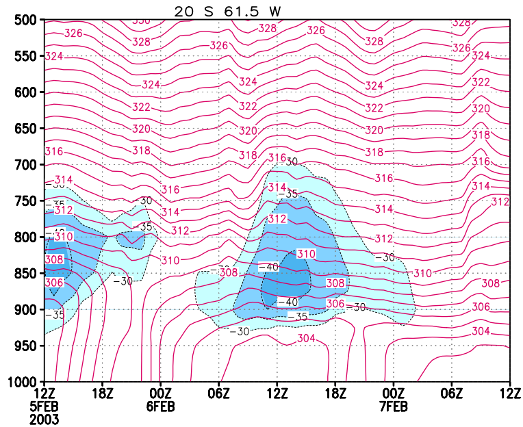
Figure 6 Time-height section of the meridional wind speed ( shaded : wind strength greater or equal to 30 kt, each 5 kt) and virtual potential temperature (contour interval 1 K) at 20° S and 61.5° W.
