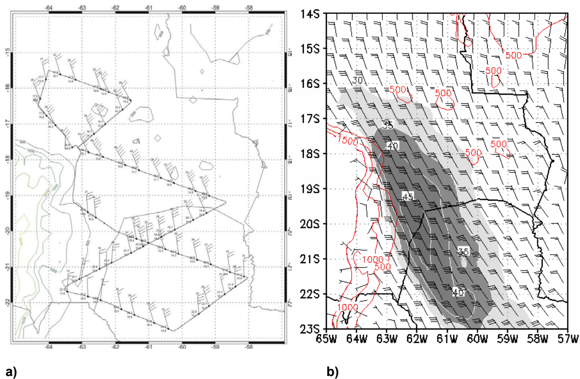
Figure 2 Observational and model simulation wind field on 6 February 2003. a) NOAA-WP-3D flight trajectory and wind field plotted at 850 hPa. (1 full barb=10 kt). b) BRAMS (1500 – 1630 UTC mean) wind field and isotach analysis (kt) at 850 hPa. Fields in mountain areas higher than 1500 m are masked.
