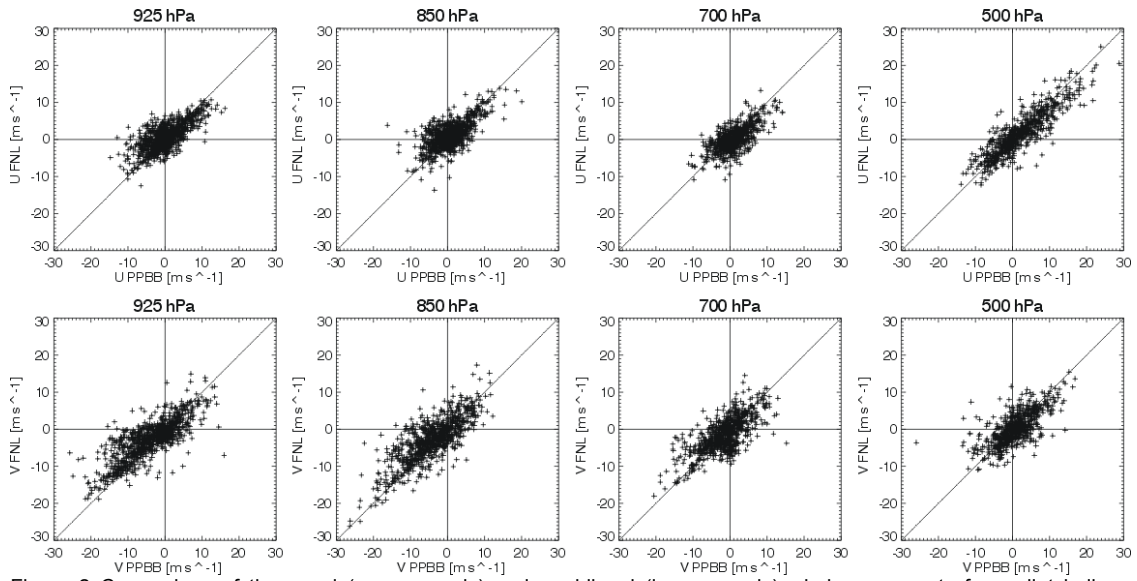
Figure 2 Comparison of the zonal (upper panels) and meridional (lower panels) wind components from pilot balloon observations and FNL analyses for different pressure levels (925, 850, 700, and 500 hPa from left to right, respectively). Scattered plots valid at 12UTC.
