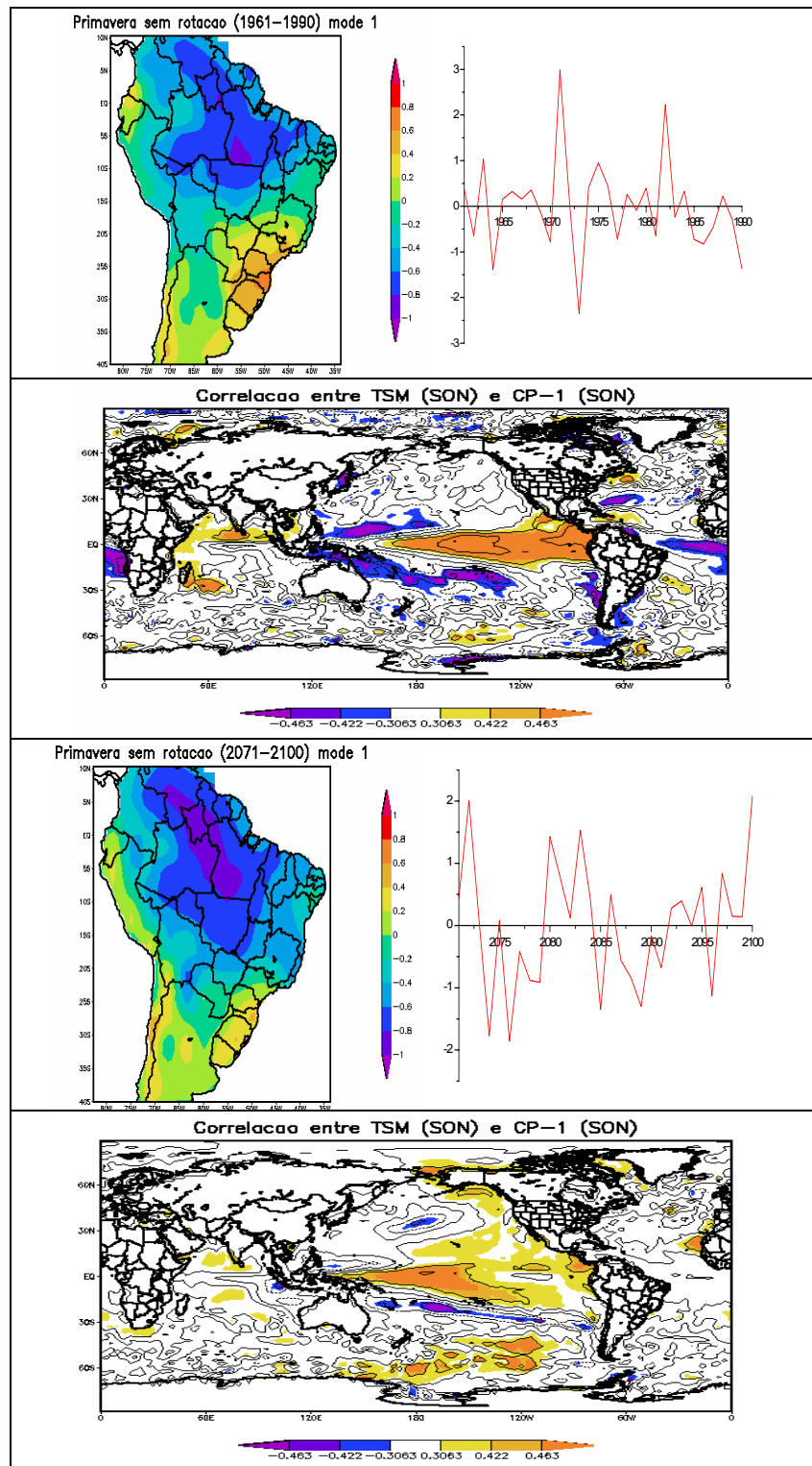
Figure 2. (Top) Factor loadings and factor scores of the first EOF of simulated spring precipitation in the period 1961-1990, and correlation coefficients between factor scores and SST. (Bottom) Same as above, for the period 2071-2100. Correlation coefficients significant to a level better than 0.05 are shaded in yellow/orange (positive) and blue/purple (negative).
