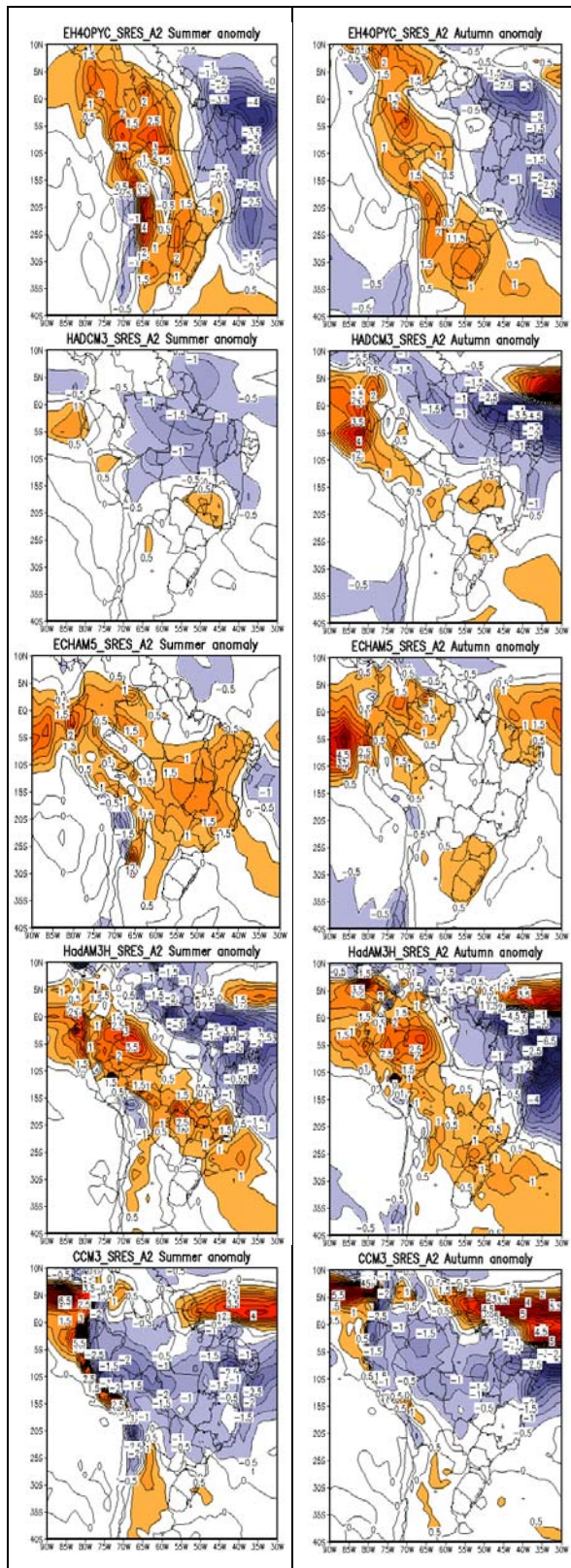
Figure 1. Climate change scenarios for summer and autumn, projected by each model included in this study (Table 1).
