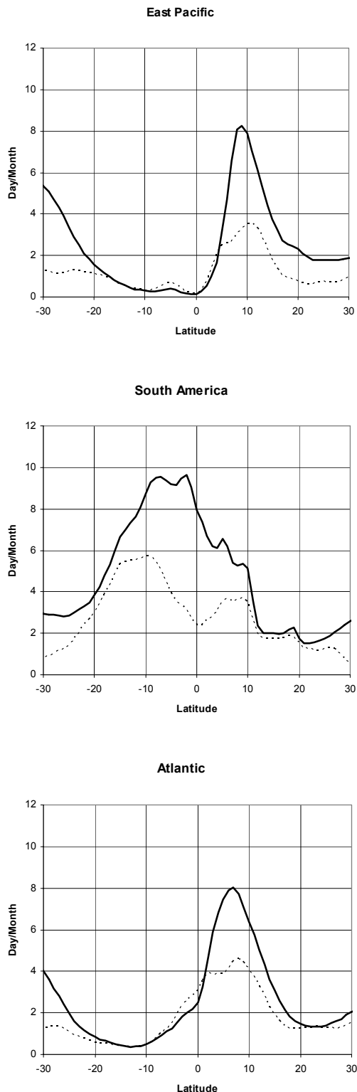
Fig. 2. Meridional profiles of convective cover occurrence for the regions given in Table 1. These profile are the zonal and temporal mean (solid lines) and standard deviation (dotted lines). The standard deviation was computed from 12 (Jan-Dec) mean monthly.
