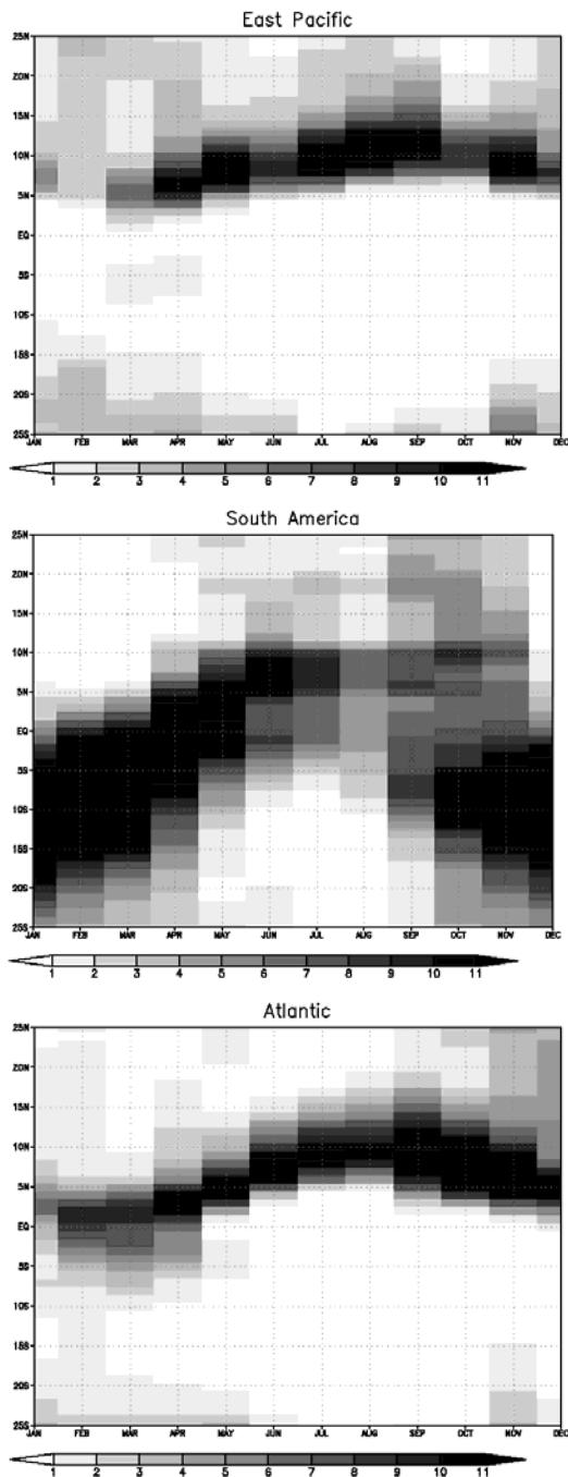
Fig. 3. Time-latitude diagrams of the mean annual cycle of ITCZ for the regions given in Table 1. The value represent a 3 years average of the number of days per month with convective cover.
