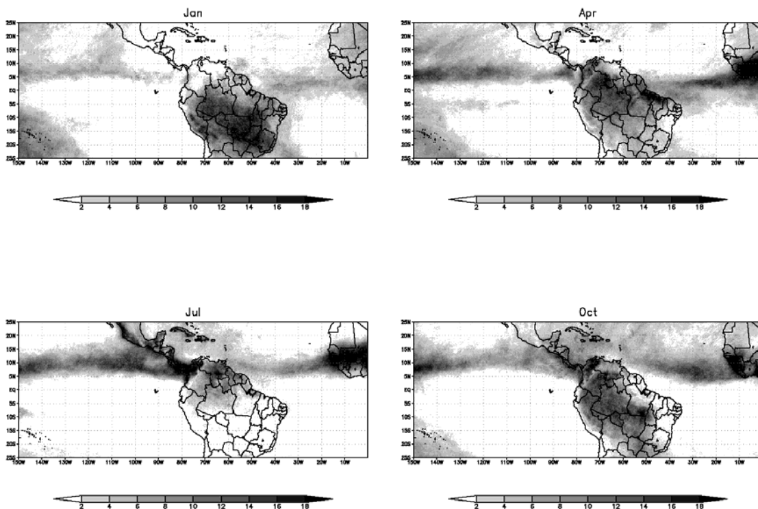
Fig. 1. Mean monthly convective cover occurrence for: (a) January, (b) April, (c) July, and (d) October. Each one were computed from the tree years 2003-2005. Value represent the number of days per month the given grid point was the infrared brightness temperature minor that 228 K.
