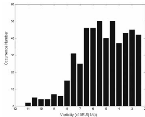
Figure 1. Number of days on which cyclonic vortices influenced NEB during austral summers of 1994 - 2001.
