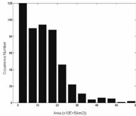
Figure 2. Number of occurrences versus the size of the cyclonic system over Northeast Brazil (NEB) in austral summers of 1994 - 2001.
