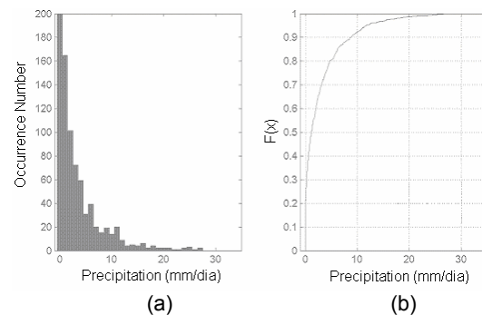
Figure 5. Frequency of occurrence of rain in the Target Area C in different classes of rainfall (mm/day) (a) and cumulative frequency (b), for December through March 1994 – 2001.
