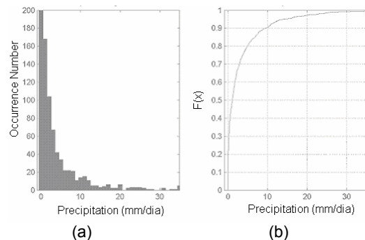
Figure 4. Frequency of occurrence of rain in the Target Area B in different classes of rainfall (mm/day) (a) and cumulative frequency (b), for December through March 1994 – 2001.
