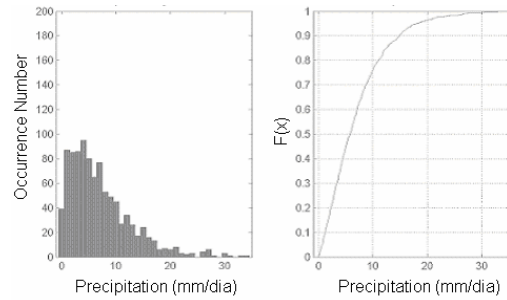
Figure 3. Frequency of occurrence of rainfall in the Target Area A in different classes of rainfall (mm/day) (a) and relative cumulative frequency (b), for the period December through March 1994 - 2001.
