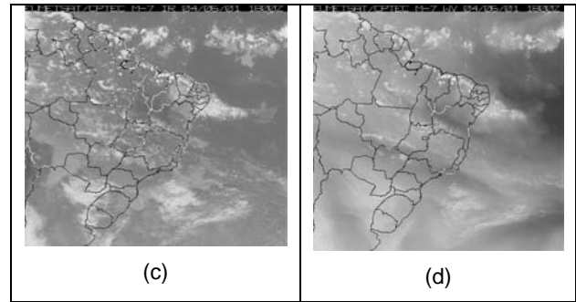
FIGURE 01 – (a) NORTHEAST BRAZILIAN REGION, SATELITE (b) VISIBLE, (c) INFRA-RED AND (d) WATER VAPOR GOES/CPTEC-INPE IMAGES.
