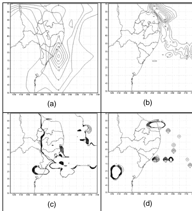
FIGURE 05 – TOTAL PRECIPITATION RATE (a) NCEP, (b) MM5 AND (c) CONVECTIVE, (b) NON-CONVECTIVE PRECIPITATION – MM5.
