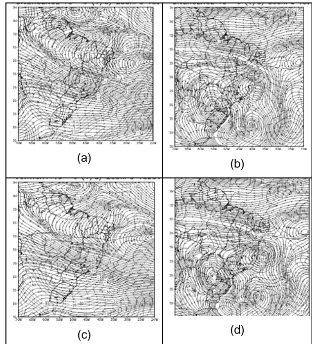
FIGURE 02 – HORIZONTAL DIVERGENCE (a) 200hPa, (b) 850hPa AND HORIZONTAL VORTICITY(c) 200hPa, (d) 850hPa – NCEP ( 10^{-6} (1/s)).
