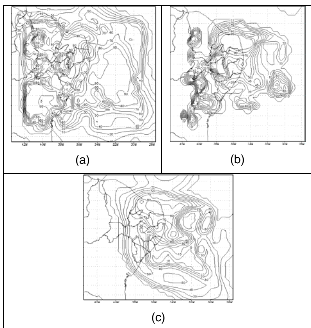
FIGURE 04 – CLOUD COVER (a) LOW, (b) MID AND (c) HIGH LEVEL -MM5.
