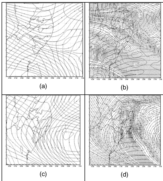
FIGURE 03 – HORIZONTAL DIVERGENCE 850 hPa (a) NCEP, (b) MM5, AND 200 hPa (c) NCEP, (d) MM5 ( 10^{-6} (1/s)).
