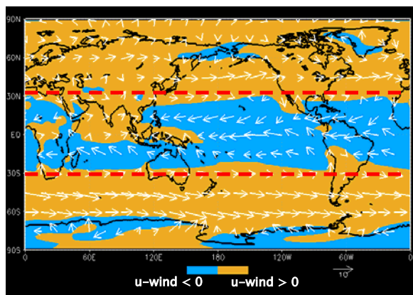
Figure 2 – Long-term average of the zonal component of low-level wind. Blue regions indicate air movement from East to West, and orange indicates air movement from West to East. Dashed red lines approximately enclose
