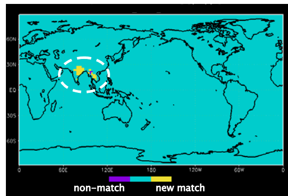
Figure 4 – Impact of the new simple fire function on the results of the CPTEC-PBM. Regions in yellow represent areas that are now correctly represented (better). Regions in blue were not affected by the new rule, and purple indicates new incorrect representation (poorer). Note that the majority of the differences indicated in Figure 1 were corrected.
