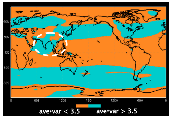
Figure 3 – Combined long-term average and intra-annual variance of the low-level zonal wind. Dashed line show regions where long-term natural fire activity due to lightning is potentially low.
