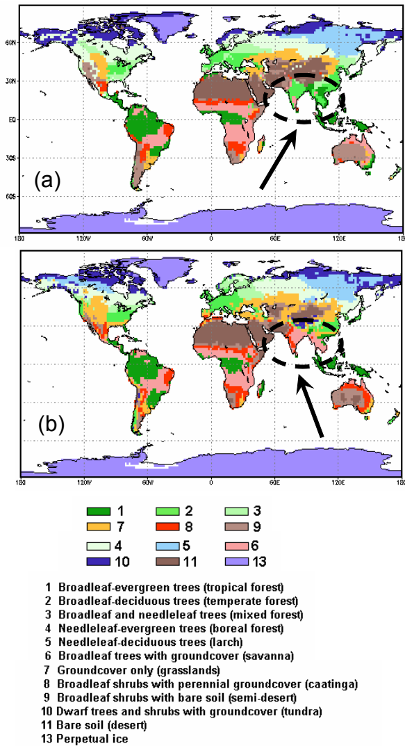
Figure 1 – Reference natural vegetation (a), and potential vegetation estimated with the CPTEC-PBM (b). Dashed lines indicate regions with important differences between the two maps.
