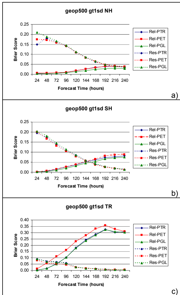
Figure 4. Average reliability and resolution components of the Brier Score for 500-hPa geopotential height forecasts. a) Northern Hemisphere; b) Southern Hemisphere; c) Tropics. Probability intervals is determined according the number of ensemble members.
