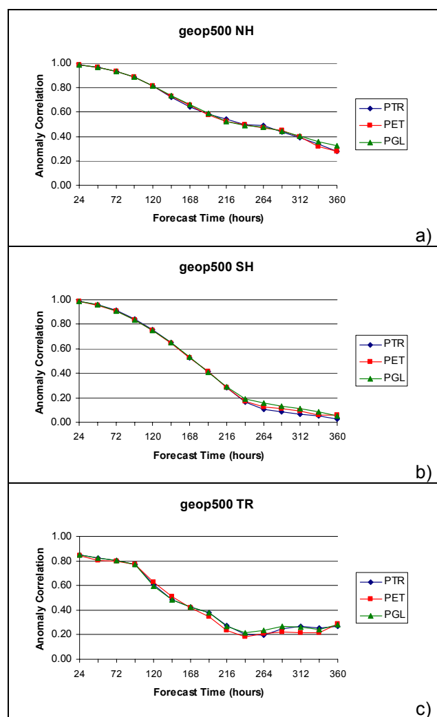
Figure 1. Average anomaly correlation of 500-hPa geopotential height ensemble mean forecasts. a) Northern Hemisphere; b) Southern Hemisphere; c) Tropics.
