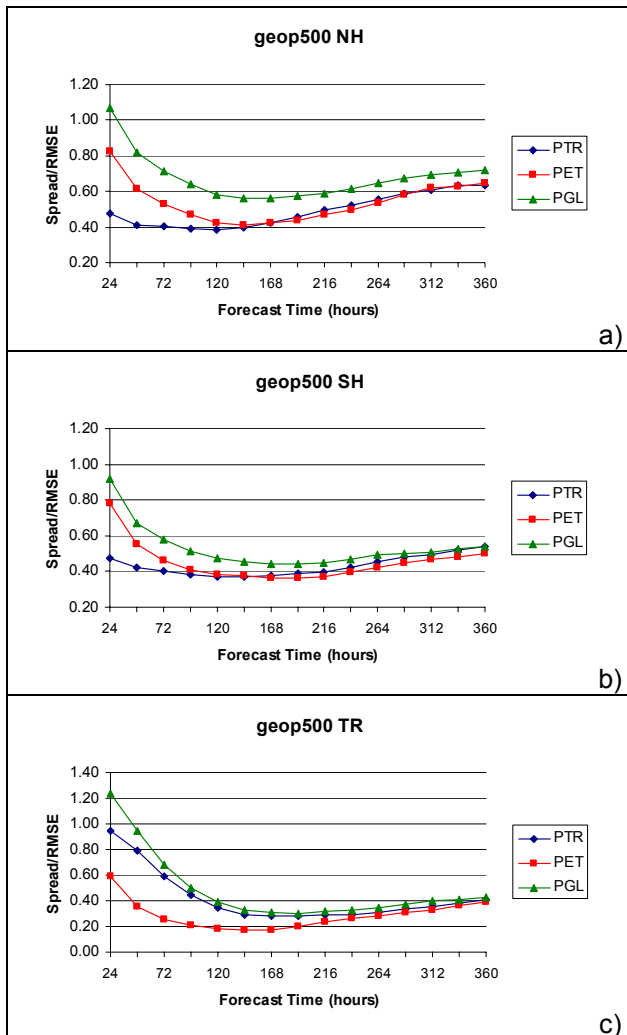
Figure 2. Average ratio of ensemble spread over RMSE of ensemble mean for 500-hPa geopotential height forecasts. a) Northern Hemisphere; b) Southern Hemisphere; c) Tropics.
