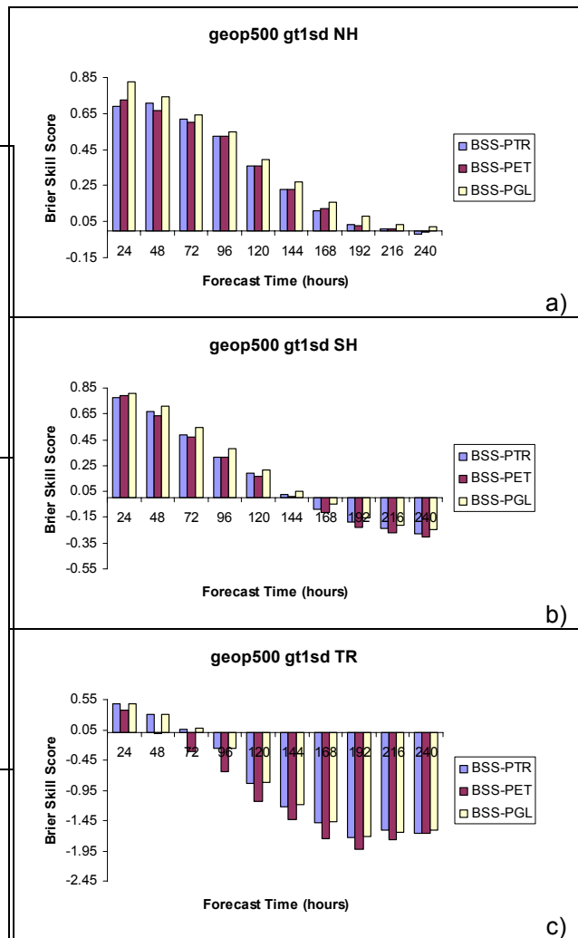
Figure 3. Average Brier Skill Score for 500-hPa geopotential height forecasts. a) Northern Hemisphere; b) Southern Hemisphere; c) Tropics. Probability intervals is determined according the number of ensemble members.
