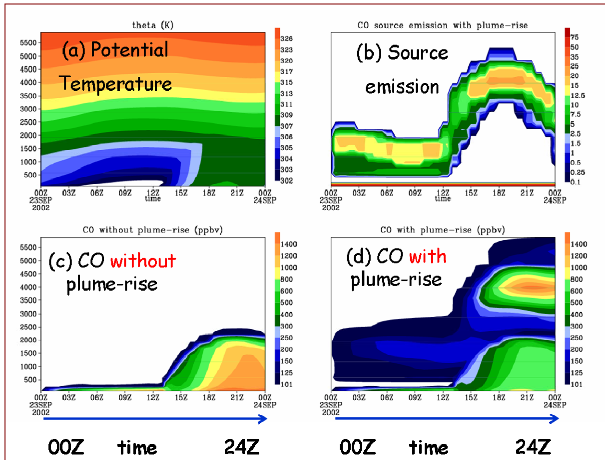
Figure 2. Diurnal cycle of the source emission with plume rise mechanism (b), the CO time evolution for a source emission without this mechanism (c) and with it (d).
