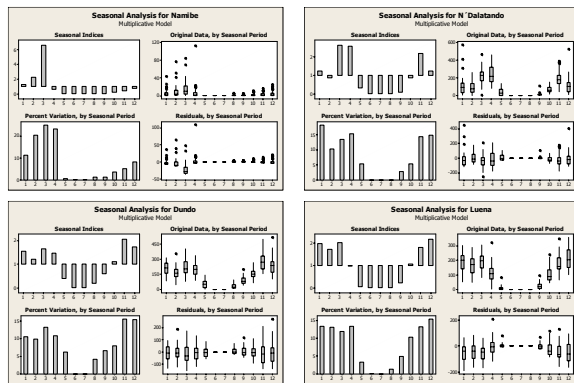
Fig.4: The monthly rainfall (1951-1980) assembling some meteorological stations. The evidence of seasonality defining the important contribution of March (3) for the rainy periods.
