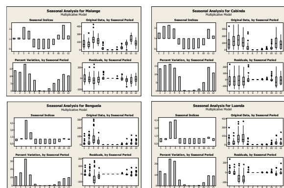
Fig.3: The monthly rainfall (1951-1980) assembling some meteorological stations. The evidence of seasonality defining the important contribution of March (3) for the rainy periods.
