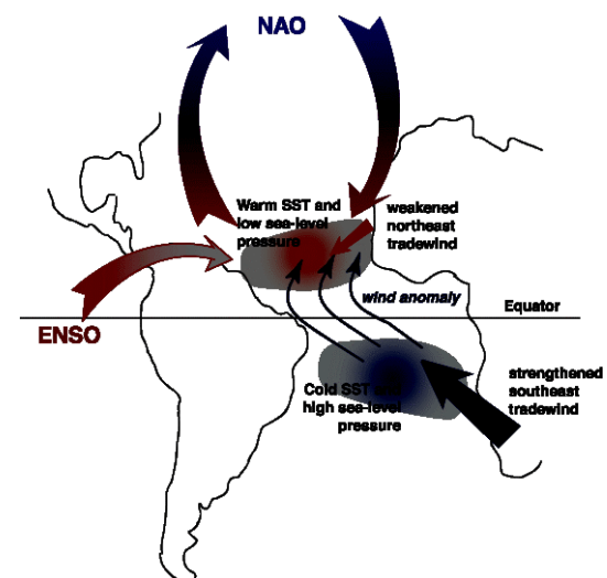
Fig.1: Revision on Planetary Circulation Configurations, which can Exert Influences in the Angola Rainfall. Source: Giannini et al., Analysis of Tropical Atlantic Variability / Preconditioning role of Tropical Atlantic Variability.
