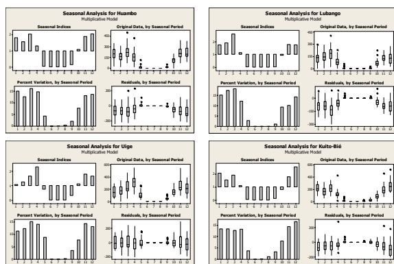
Fig.5: The monthly rainfall (1951-1980) assembling some meteorological stations. The evidence of seasonality defining the important contribution of March (3) for the rainy periods.
