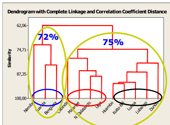
Cluster 1 (Similarity = 81.55%) HUAMBO; KUITO-BIÉ; LUENA; LUBANGO; DUNDO. Cluster 2 (Similarity = 79.12%) UIGE; N'DALATANDO; MALANGE; CABINDA. Cluster 3 (Similarity = 72.05%) BENGUELA; LUANDA; NAMIBE.
