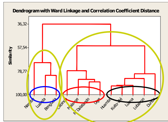
Cluster 1 (Similarity = 81.20%) HUAMBO; KUITO-BIÉ; LUENA; LUBANGO; DUNDO. Cluster 2 (Similarity = 78.28%) UIGE; N'DALATANDO; MALANGE; CABINDA. Cluster 3 (Similarity = 71.02%) BENGUELA; LUANDA; NAMIBE.
