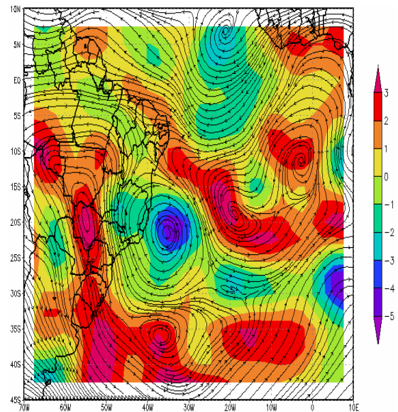
Figure 5- Stream lines (black lines) and relative vorticity ( \times 10^{-5} \text{s}^{-1} , colours) at 600hPa level, 14 August, 2004, 12UTC. Source: NCEP.
