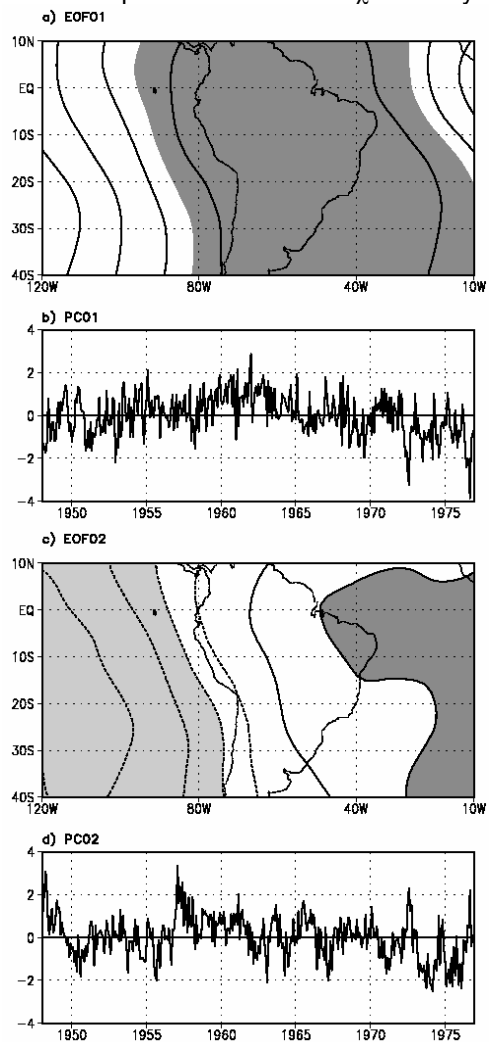
Figure 1 – Loading patterns and PC of the first two EOF modes of the transient- \chi for 1948-1976. Contour interval is 0.20. The zero contour has been omitted. Light (Dark) shading area indicates values less (greater) than -0.7 (0.7) in (a) and than -0.4 (0.4) in (c).
