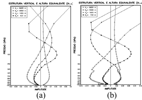
Fig. 3 – Vertical structures, correspondig to equivalent height Hn for the CPTEC Global Model: (a) 28 and (b) 42 levels.
