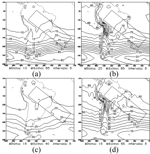
Fig. 4- Total energy (%), NCEP Analyses T126L28 (top) and T170L42 (bottom): (a) and (c) 1 st to 3 rd , (b) and (d) 4 th to 7 th vertical modes.
