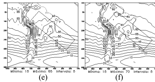
Fig. 9- Total energy (%) of the vertical modes, CPTEC Global Model T126L28 (left) and T170L42 (right): (a) and (b) Kuo; (c) and (d) RAS; (e) and (f) Grell deep convection schemes.
