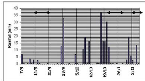
Figure 1- Time series of rainfall at the pasture site during LBA-RACCI 2002 in Rondonia.
