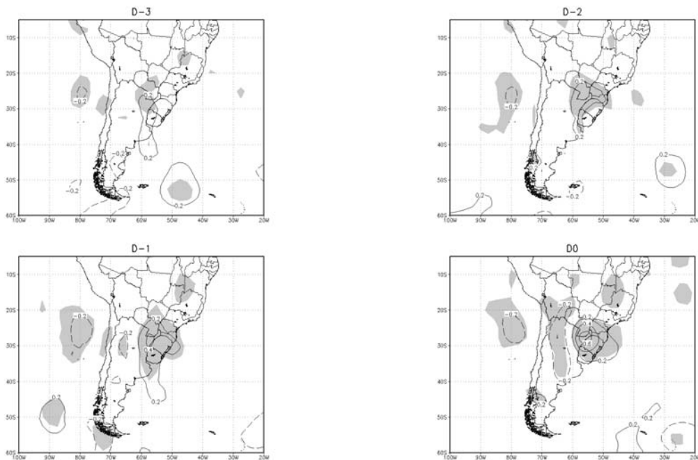
Figure 8: Same as in Fig. 4, except for the 850-hPa horizontal thermal advection ( 10^{-4} \text{ K s}^{-1} ).
