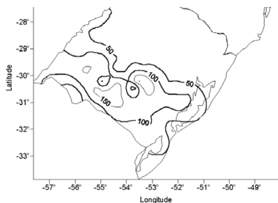
Figure 2: Isohyet analysis of a typical heavy rainfall episode. This episode occurred on 12 april 1992 in which there was heavy and widesread rainfall.
