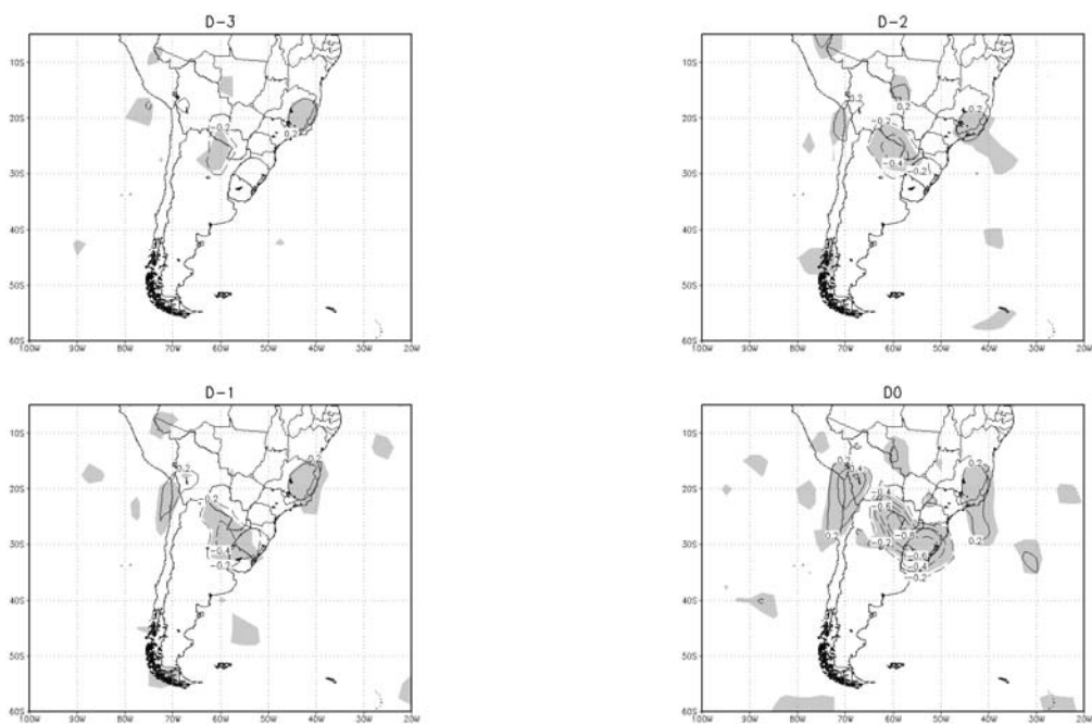
Figure 7: Same as in Fig. 4, except for the 850-hPa divergence of water vapor flux ( 10^{-7} \text{ s}^{-1} ).
