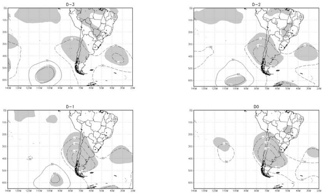
Figure 4: 500-hPa geopotential height (m) anomaly composites for the 41 heavy rainfall episodes in autumn season (MAM), in southern Brazil. The shaded areas show significance at the 95% level.
