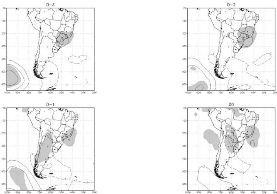
Figure 5: Same as in Fig. 4, except for the sea-level pressure anomaly (hPa).
