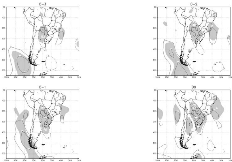
Figure 6: Same as in Fig. 4, except for the 850-hPa meridional wind component ( \text{m s}^{-1} ).
