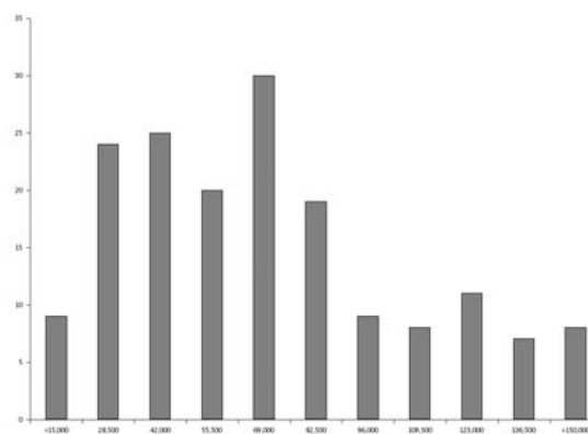
Figure 3: Frequency distribution of heavy rainfall episodes in southern Brazil based on the area enclosed by 50\text{-mm day}^{-1} isohyet ( A_{50} ) in the 1991-2001 period. The ordinate shows the frequency of heavy rainfall episodes in each 50\text{-mm day}^{-1} class indicated in the abscissa on \text{km}^2 .
