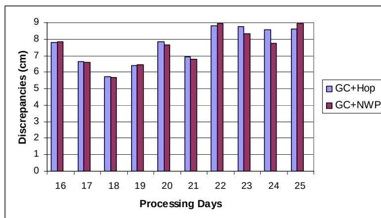
Figure 3. Discrepancies obtained in PPP with different troposphere models
