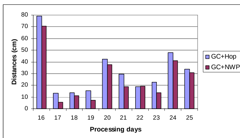
Figure 4. Distance obtained in relative positioning with different troposphere models
